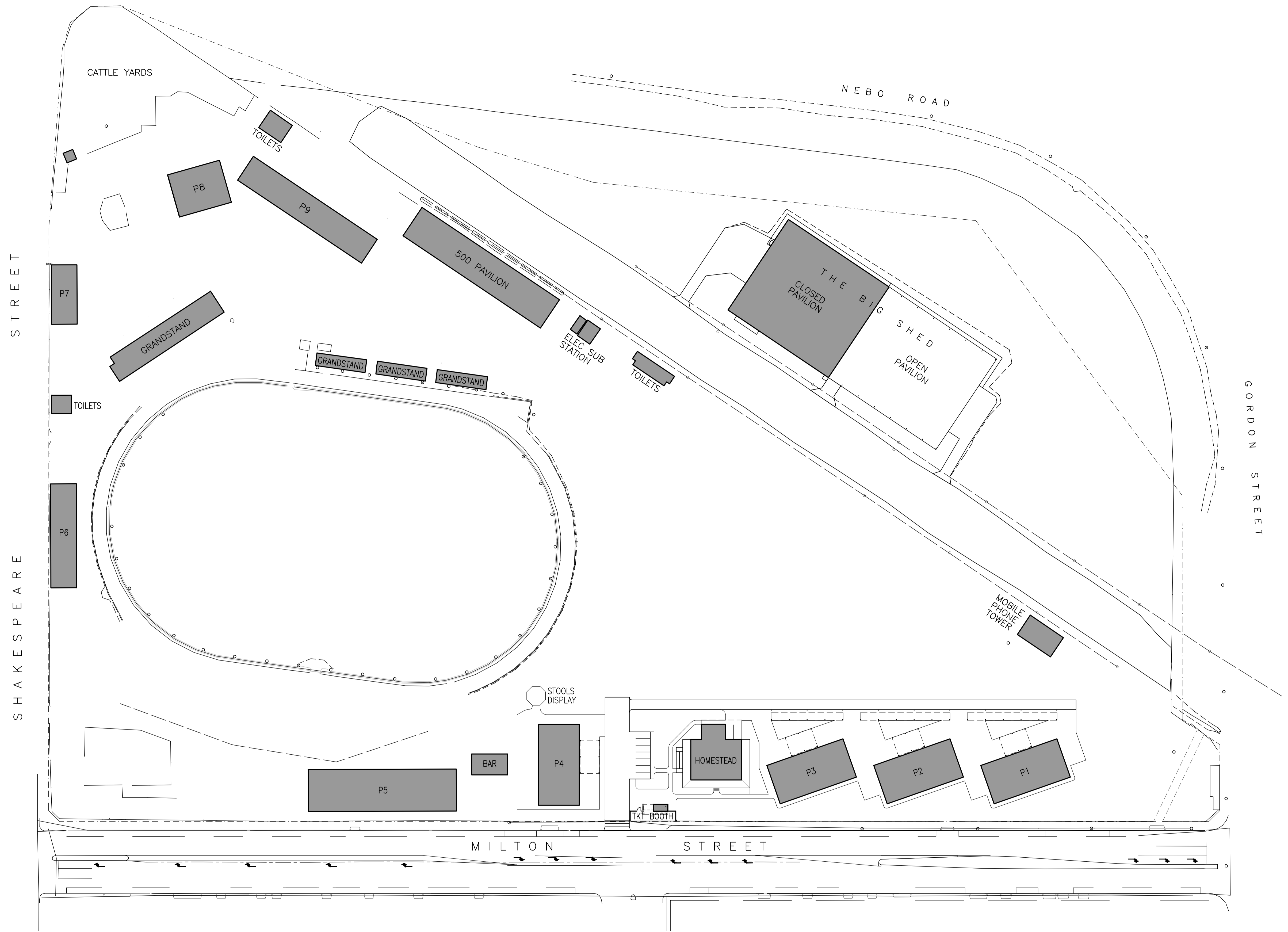
1 SITE PLAN SCALE 1:750
